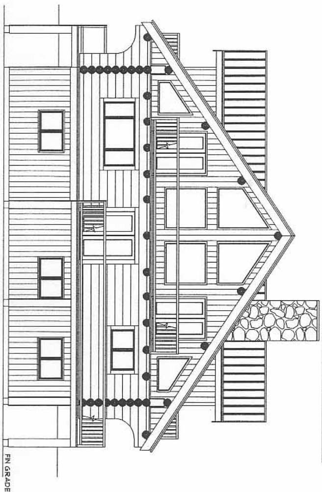
REAR ELEVATION
