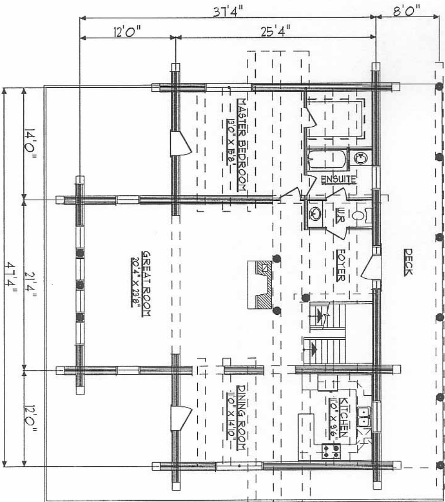
MAIN FLOOR PLAN 512.96 FT
