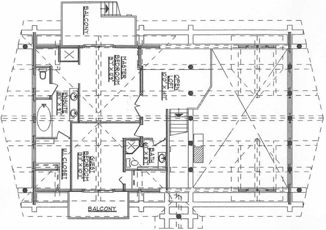
LOFT FLOOR PLAN 906 SF
