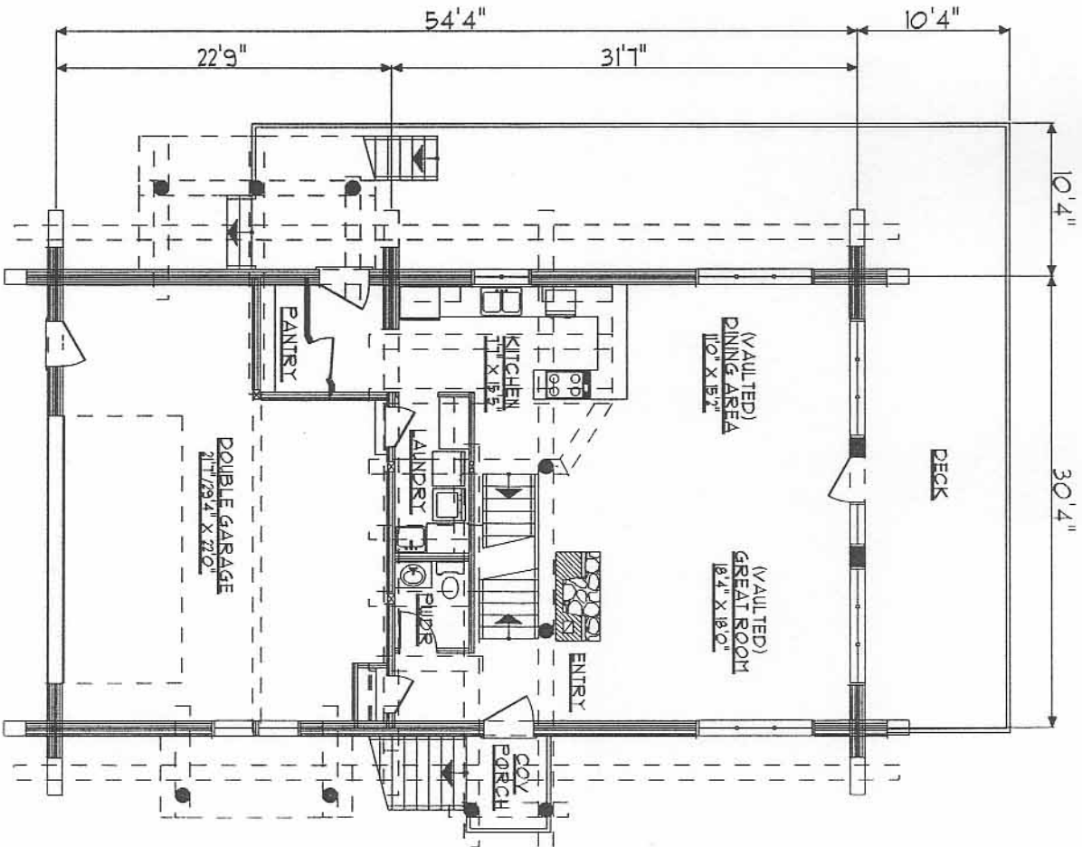
MAIN FLOOR PLAN 1001 SF 518 SF GARAGE
