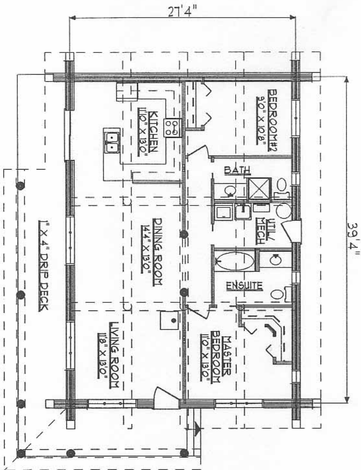
MAIN FLOOR PLAN 120 SE
